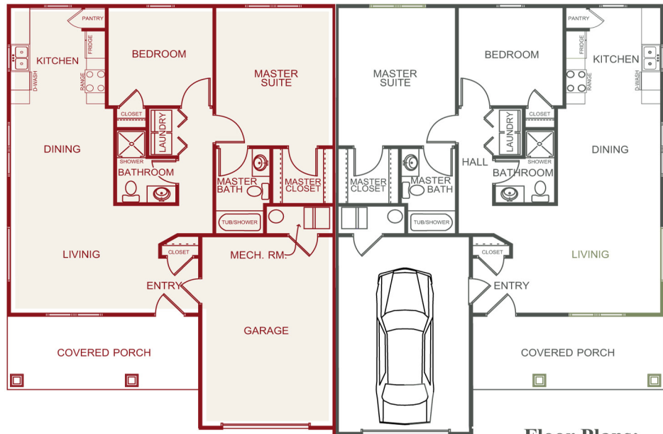
Floor Plans: Approx. 1,146 sq.ft.
